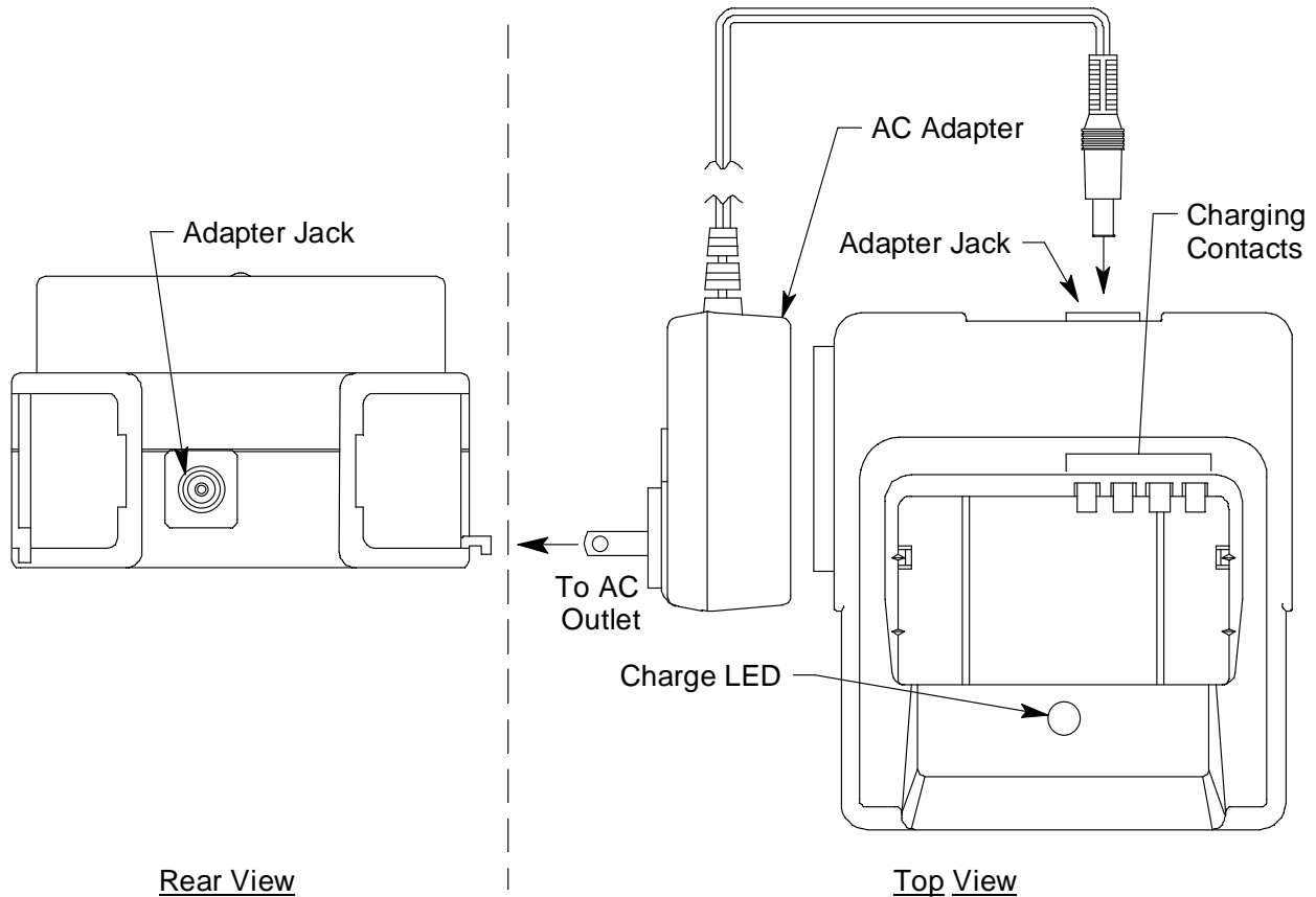
Figure 5: GX-212 AC Powered Charging Station
